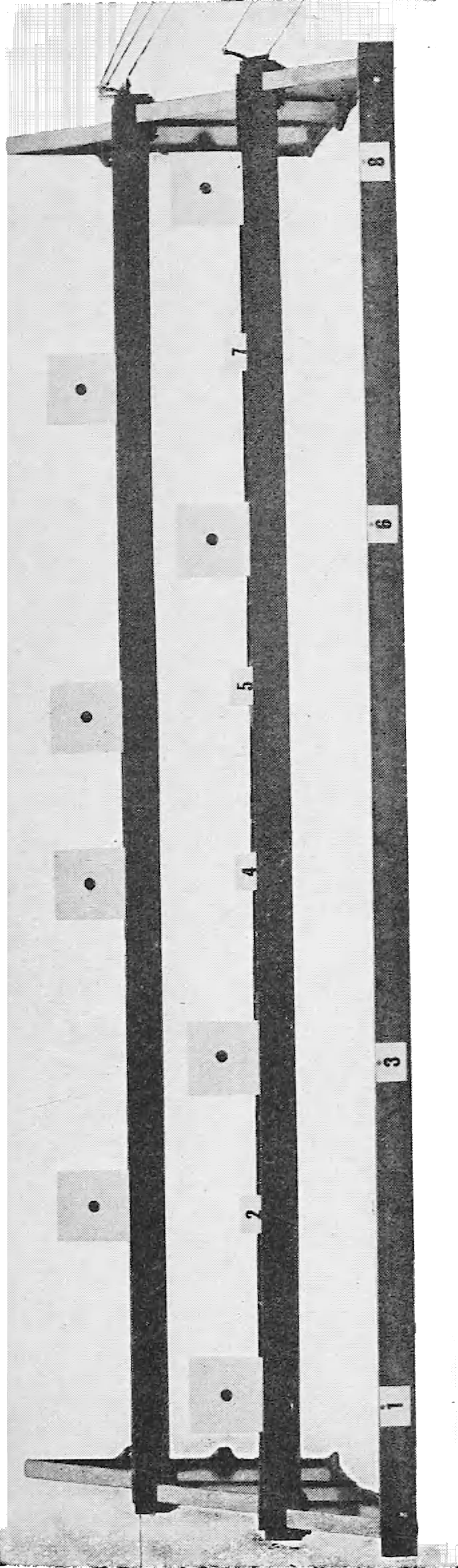
Fig. 53. —SOLANO TARGET, MARK I, ARRANGED FOR ELEMENTARY PRACTICES. (See Appendix, Sec. VII., para. 2.)
